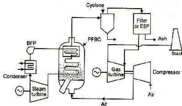
Figure: PFBC turbocharged arrangement
