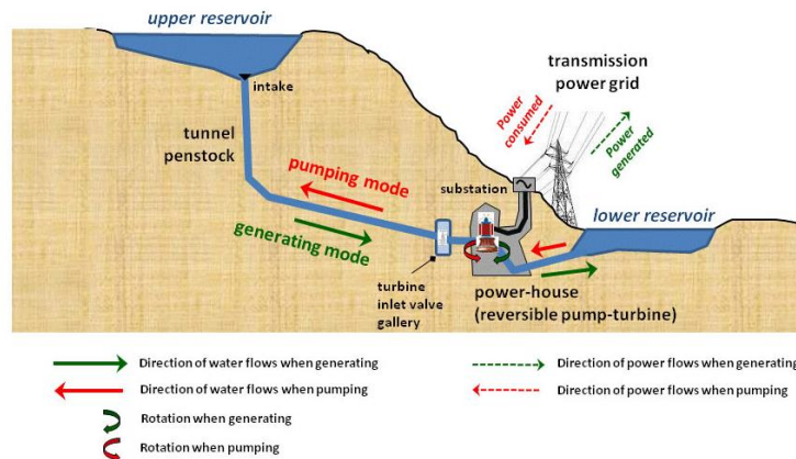
Figure: Pumped storage plant.
