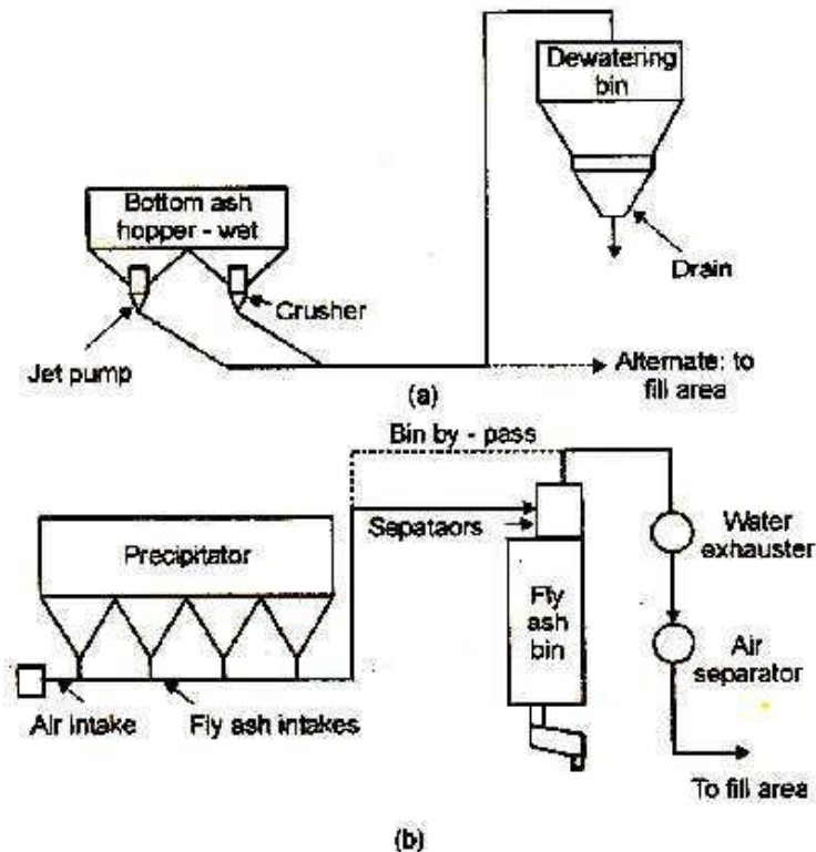
Figure: Layout of ash handling system.
