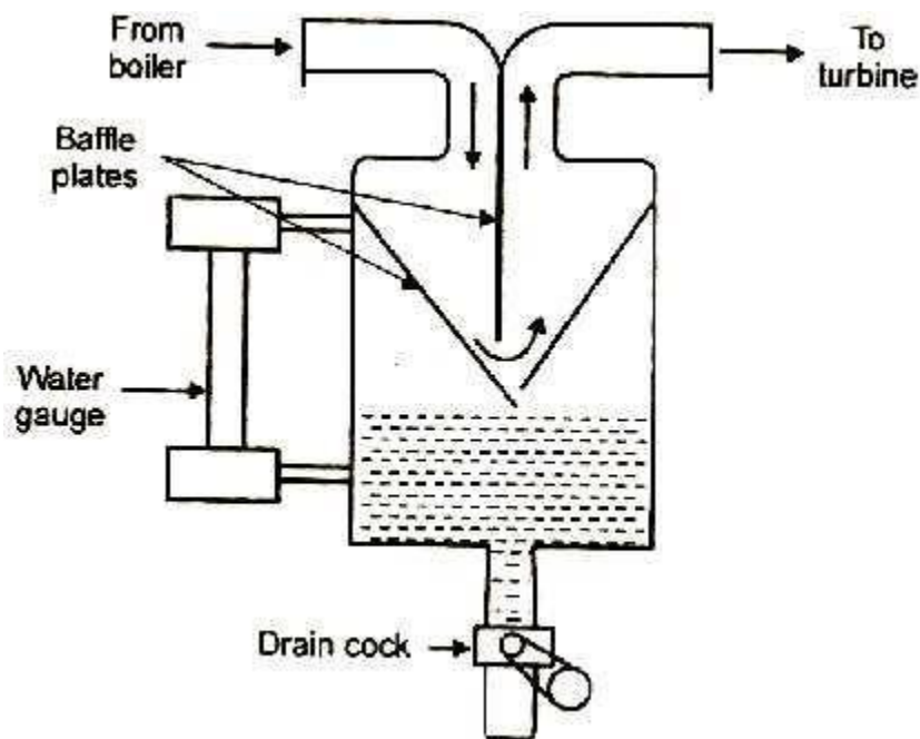
Figure: Steam separator
