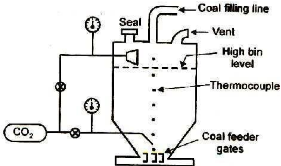
Figure : Control system used for storing the pulverized coal with the use of CO 2 .
