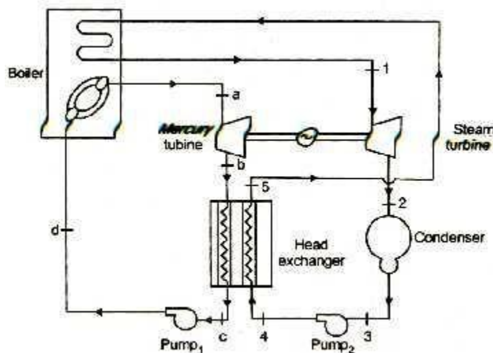
Figure: Mercury-steam binary vapor cycle
