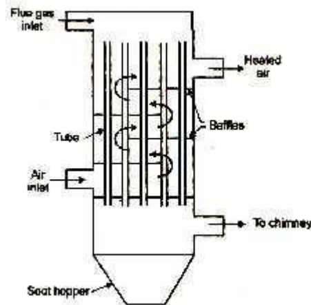
Figure: Air pre-heater
