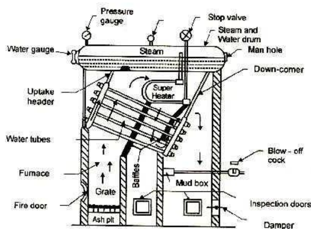
Figure: Babcock and Wilcox boiler
