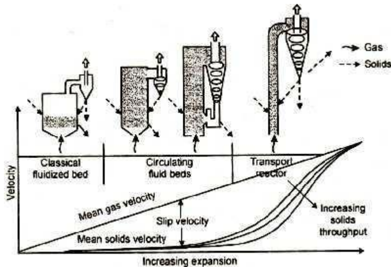
Figure: Basic fluid bed Systems
